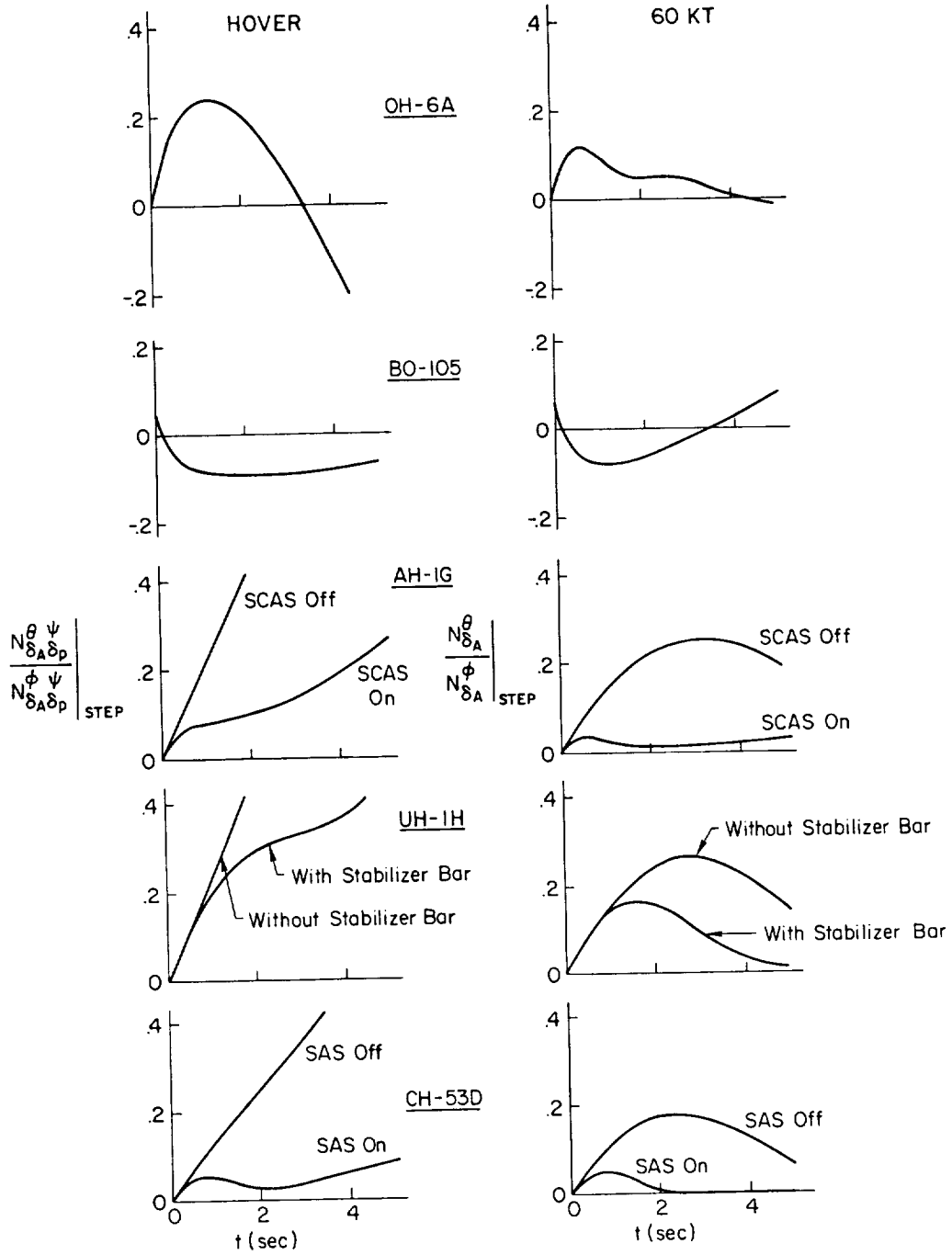
Figure III-14. \phi_c \rightarrow \theta Cross Coupling Effect
